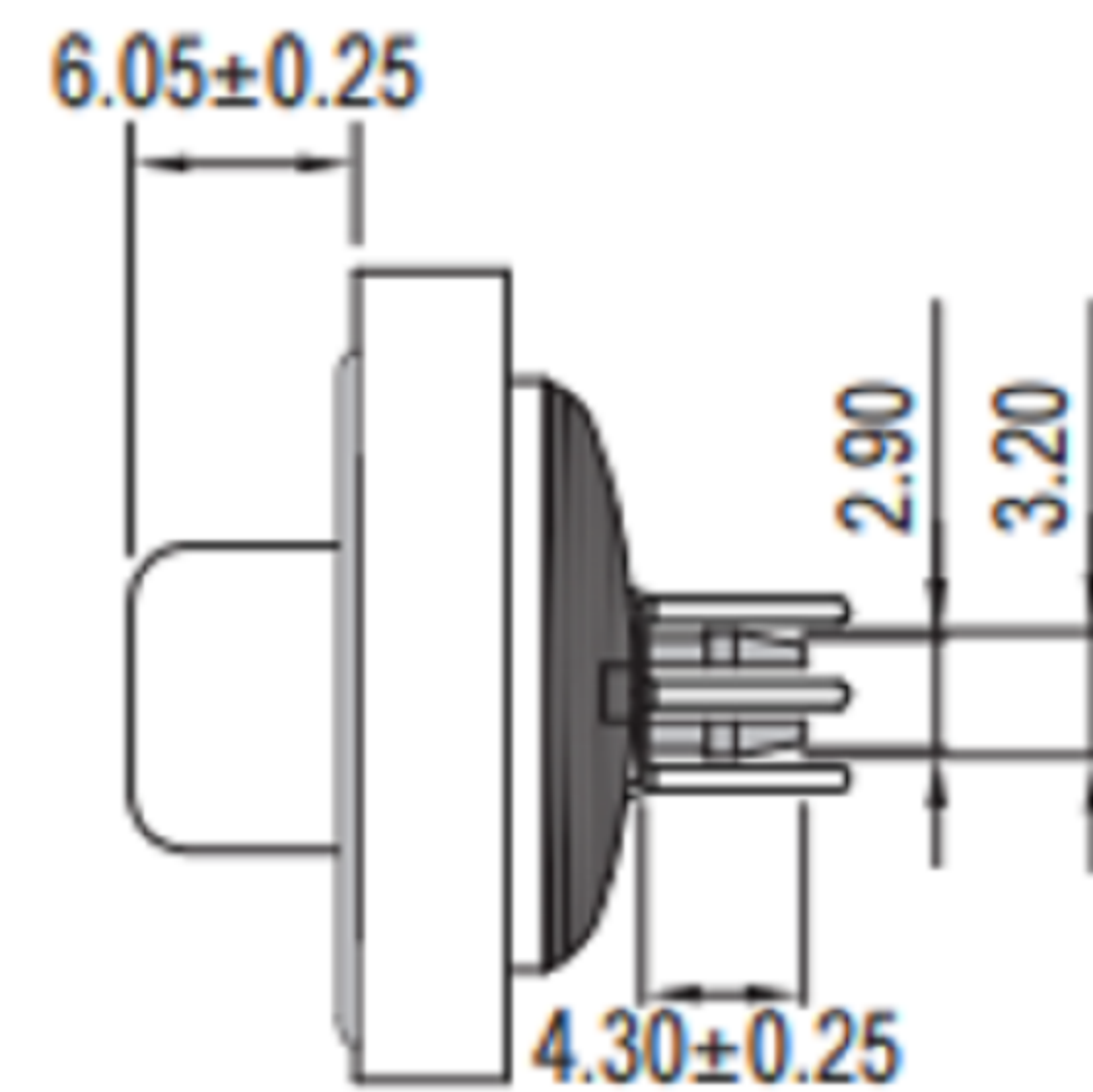
直式针型插座(焊板式, 定位柱) EDB4 Straight Male Socket(PCB, Peg) EDB4 - M 37 - PPA 14 - DW
